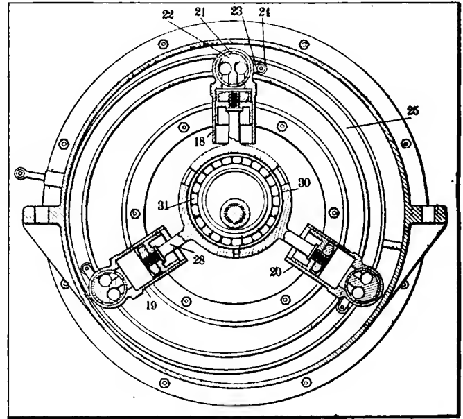
Fig. 2.—Mounting of driven pumps—Section B B in Fig. 1
